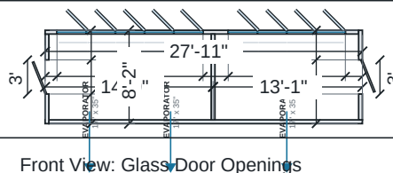
Front View: Glass Door Openings
