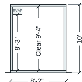
Side Section (Clear Height)
