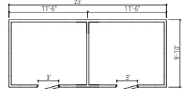
CMB10X23-12C11F-36R36L
