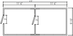
CMB10X23-12C11F-36L36L
