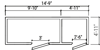
CMB5X15-10C5F-36R30CR
