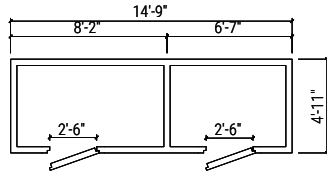
CMB5X15-8C7F-30R30R
