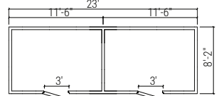
CMB8X23-12C11F-36L36L
