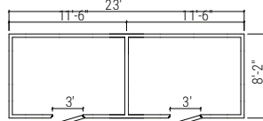
CMB8X23-12C11F-36R36R
