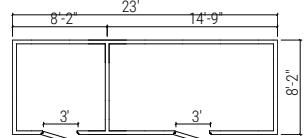
CMB8X23-15C8F-36L36L
