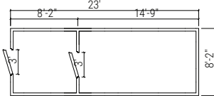
CMB8X23-15C8F-36R36R
