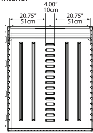
6051XL Interior
