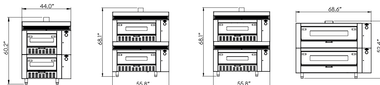
FRONT VIEW
