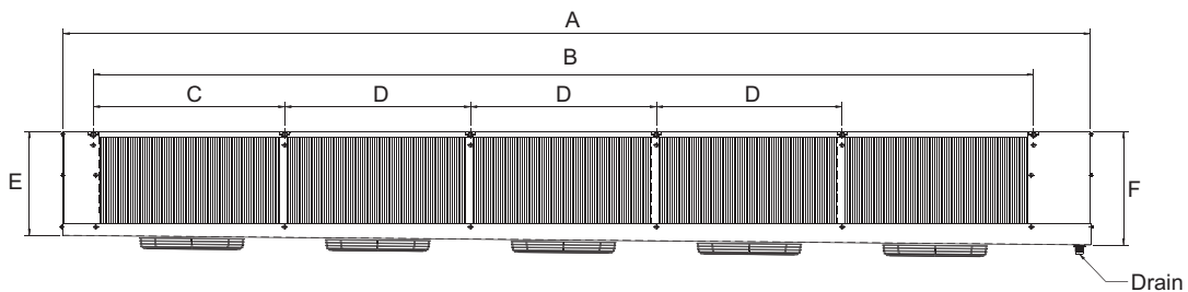
FRONT VIEW
